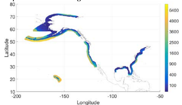
FIGURE 1. GEOGRAPHIC DISTRIBUTION OF PARTITION DATA. COLORS REPESENT WATER DEPTH (M).
