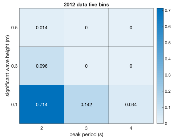
FIGURE 2 - JOINT PROBABILITY DISTRIBUTION LAKE WASHINGTON
