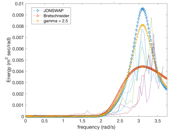
FIGURE 3 - ESTIMATING GAMMA FOR LAKE WASHINGTON SPECTRA, 0.3M H_s , 2s T_p WAVE CASE
