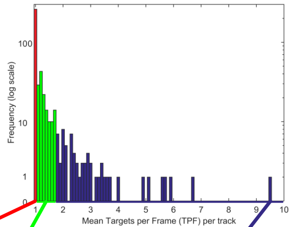
FIGURE 3. THE MEAN TPF OVER A TRACK CAN BE USED TO CLASSIFY MULTIBEAM TARGETS INTO 'SINGLE TARGETS' (A), 'SMALL SCHOOLS' (B) AND 'LARGE SCHOOLS' (C). SINGLE TARGETS CAN BE FURTHER CLASSIFIED INTO FISH, DIVING BIRDS DISTINGUISHED BY THEIR CHARACTERISTIC U-SHAPED DIVE [13] AS SHOWN HERE AND MARINE MAMMALS CHARACTERIZED BY THEIR LARGE SIZE. EXAMPLE TARGETS ARE AVERAGED OVER SEVERAL SECONDS TO HIGHLIGHT MOVEMENT AND ARE FROM THE 2013 DEPLOYMENT ADJACENT TO THE ATLANTIS AK-1000 TURBINE STRUCTURE. THE TURBINE STRUCTURE IS SHADED IN GREEN, AND THE EXPECTED BLADE RADIUS IS OUTLINED BY A DASHED GREEN LINE. RANGES ARE IN METERS.
